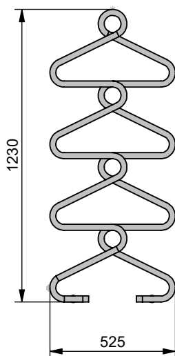
Front view ABZ/ABZC-120-50
